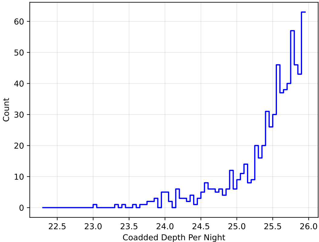
noroll_mjdp180_v3.4_10yrs u band: DD:WFD CoaddM5PerNight
