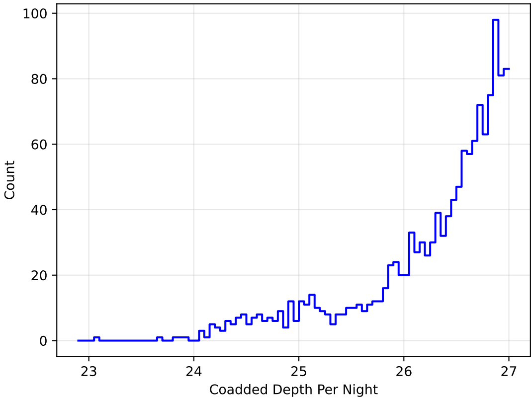
noroll_mjdp180_v3.4_10yrs r band: DD:WFD CoaddM5PerNight
