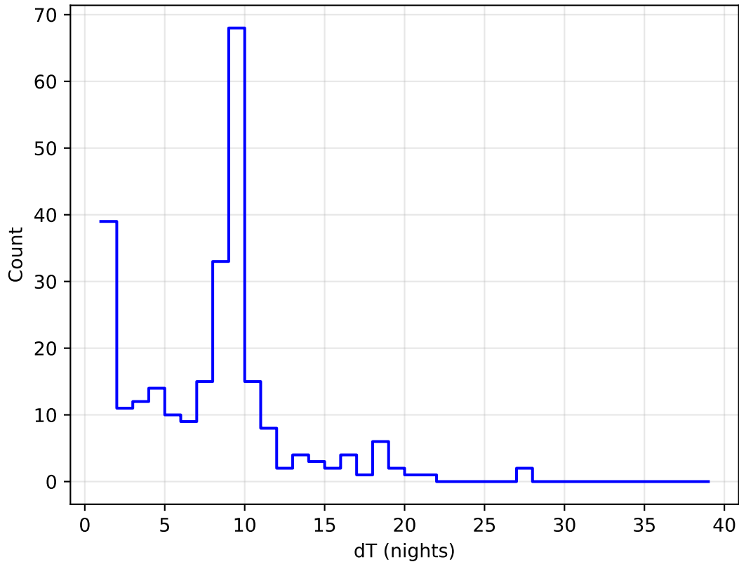
noroll_mjdp180_v3.4_10yrs all bands: DD:ELAISS1 Delta Nights Histogram
