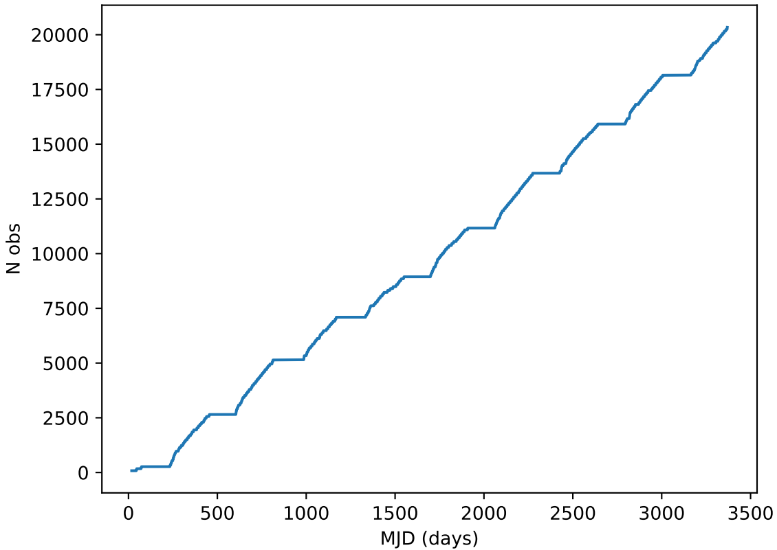
noroll_mjdp180_v3.4_10yrs all bands: DD:ELAISS1 Cumulative NVisits
