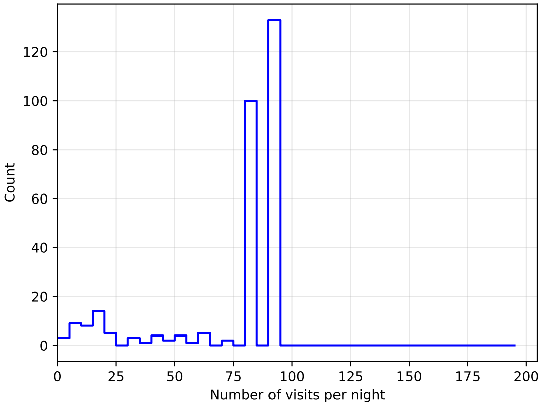
noroll_mjdp180_v3.4_10yrs all bands: DD:EDFS NVisitsPerNight
