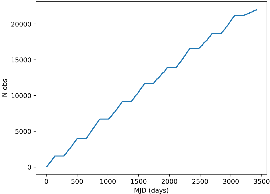
noroll_mjdp180_v3.4_10yrs all bands: DD:EDFS Cumulative NVisits
