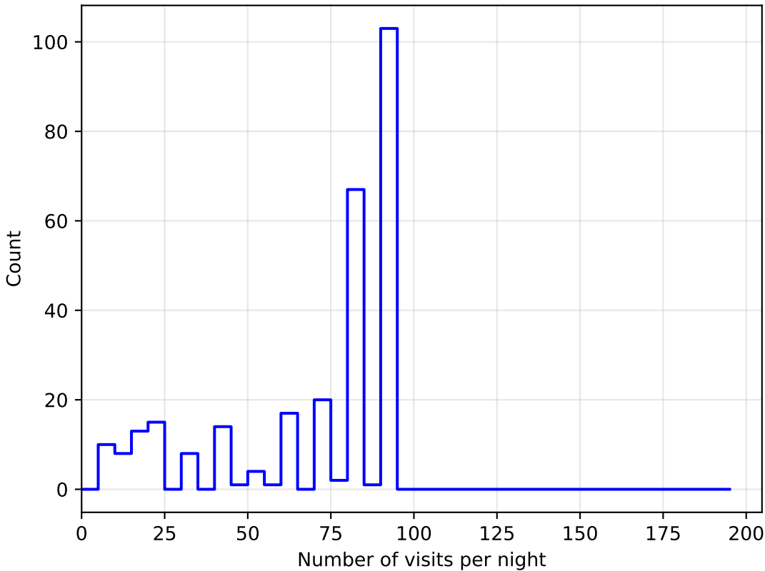
noroll_mjdp180_v3.4_10yrs all bands: DD:ECDFS NVisitsPerNight
