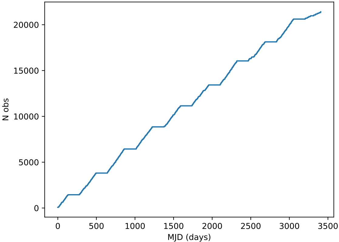
noroll_mjdp180_v3.4_10yrs all bands: DD:ECDFS Cumulative NVisits
