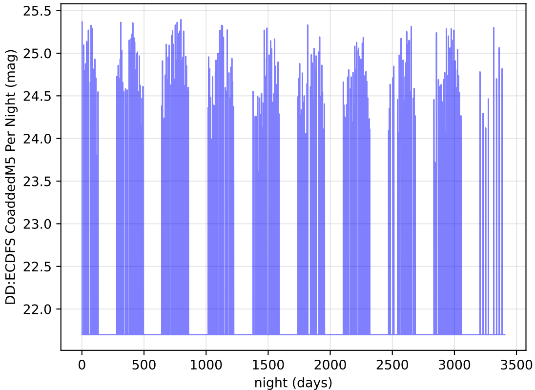
noroll_mjdp180_v3.4_10yrs z band: DD:ECDFS CoaddedM5 Per Night
