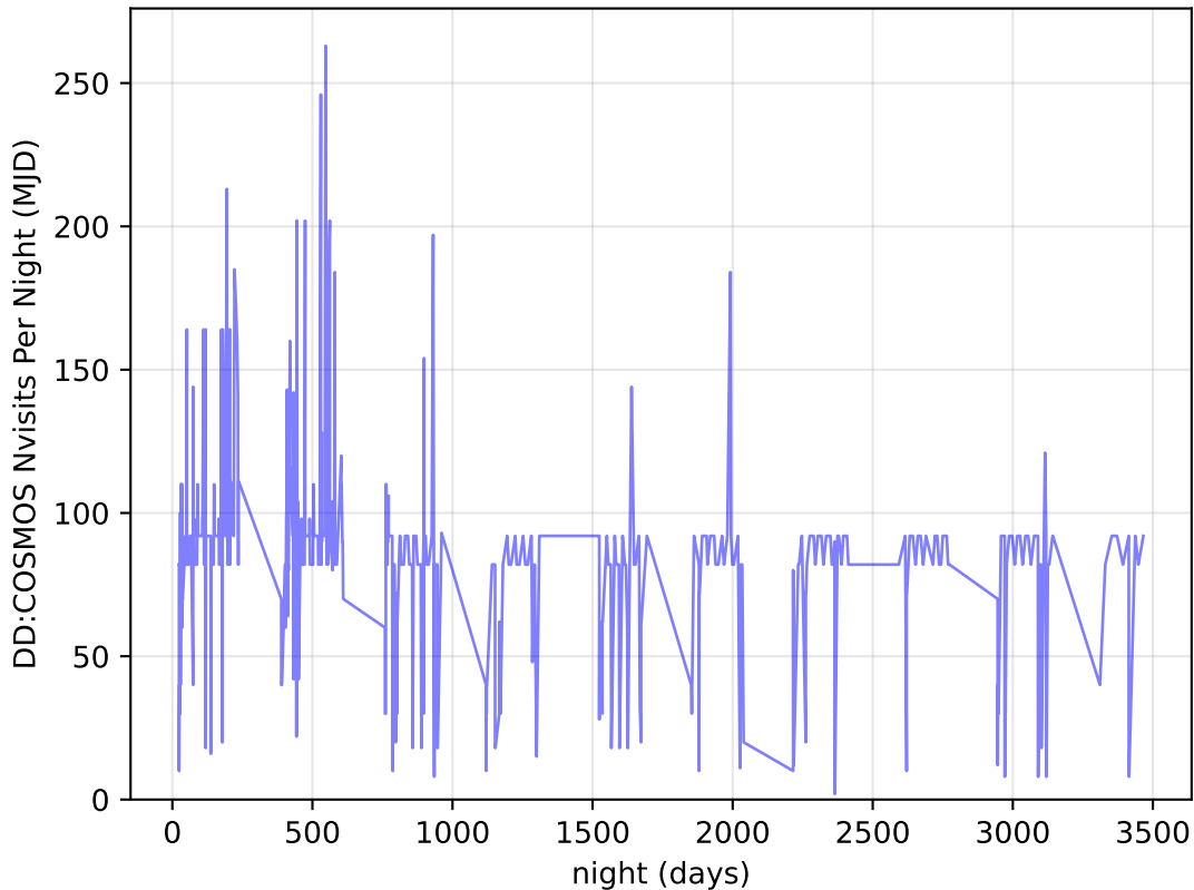
noroll_mjdp180_v3.4_10yrs all bands: DD: COSMOS Nvisits Per Night
