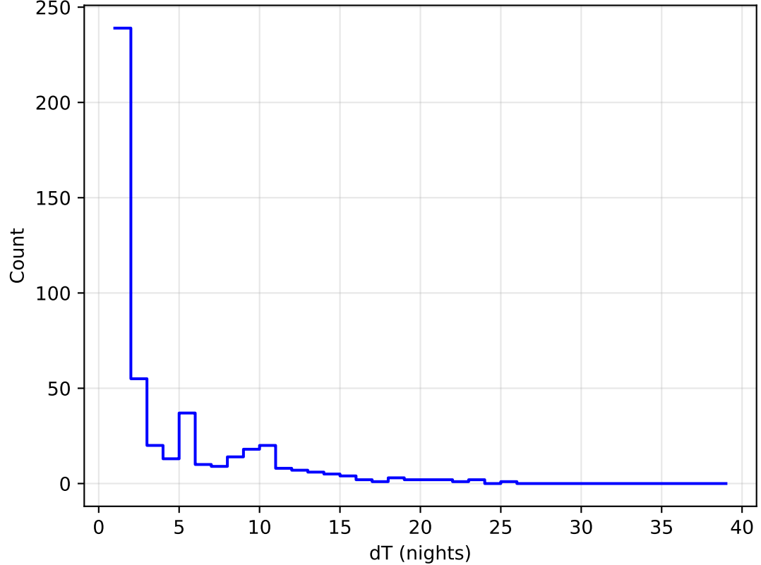
noroll_mjdp180_v3.4_10yrs all bands: DD: COSMOS Delta Nights Histogram
