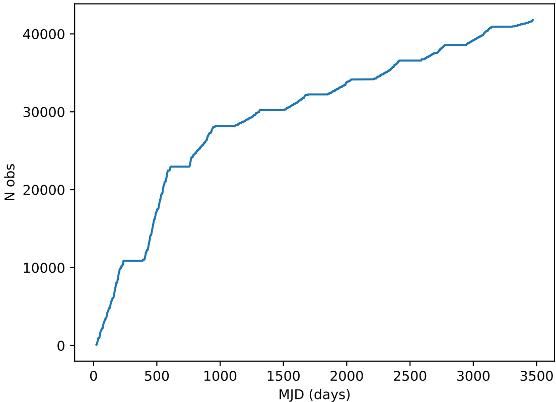
noroll_mjdp180_v3.4_10yrs all bands: DD:COSMOS Cumulative NVisits
