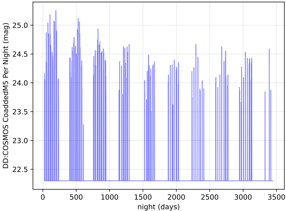
noroll_mjdp180_v3.4_10yrs u band: DD:COSMOS CoaddedM5 Per Night
