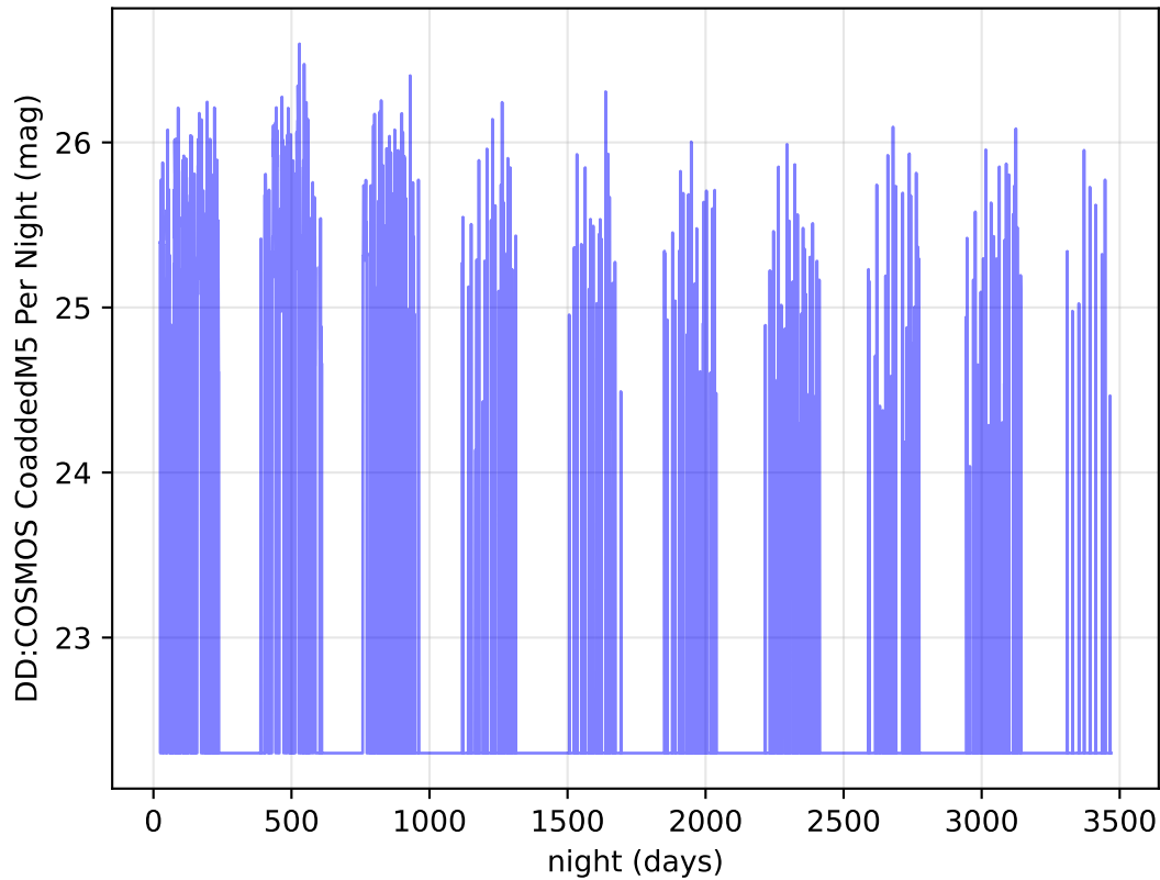
noroll_mjdp180_v3.4_10yrs g band: DD:COSMOS CoaddedM5 Per Night
