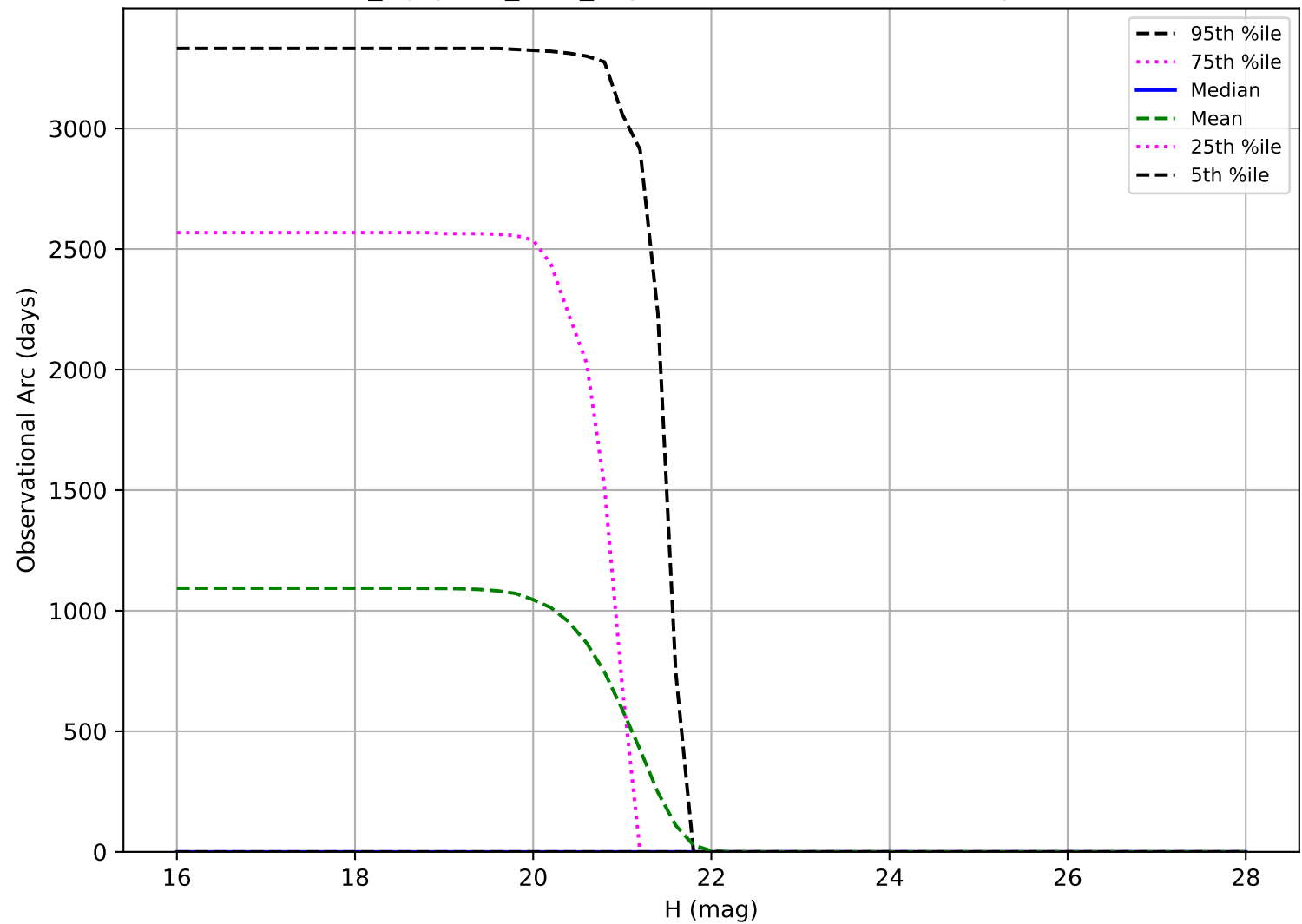
noroll_mjdp120_v3.4_10yrs: Observational Arc Length Vatira
