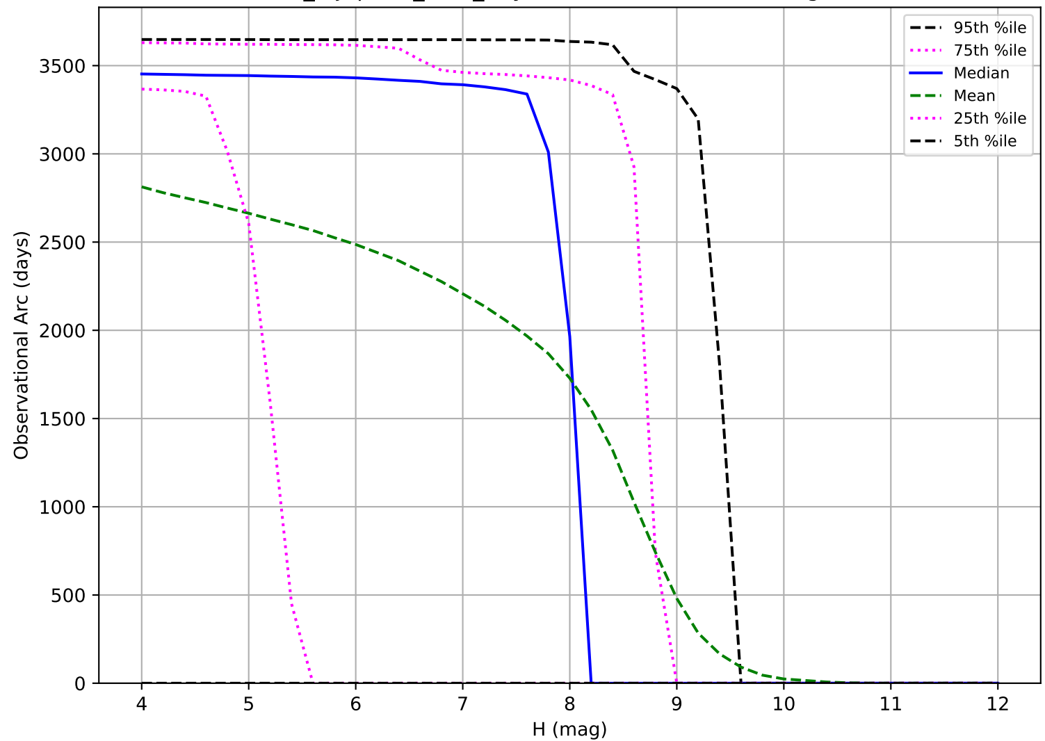
noroll_mjdp120_v3.4_10yrs: Observational Arc Length TNO
