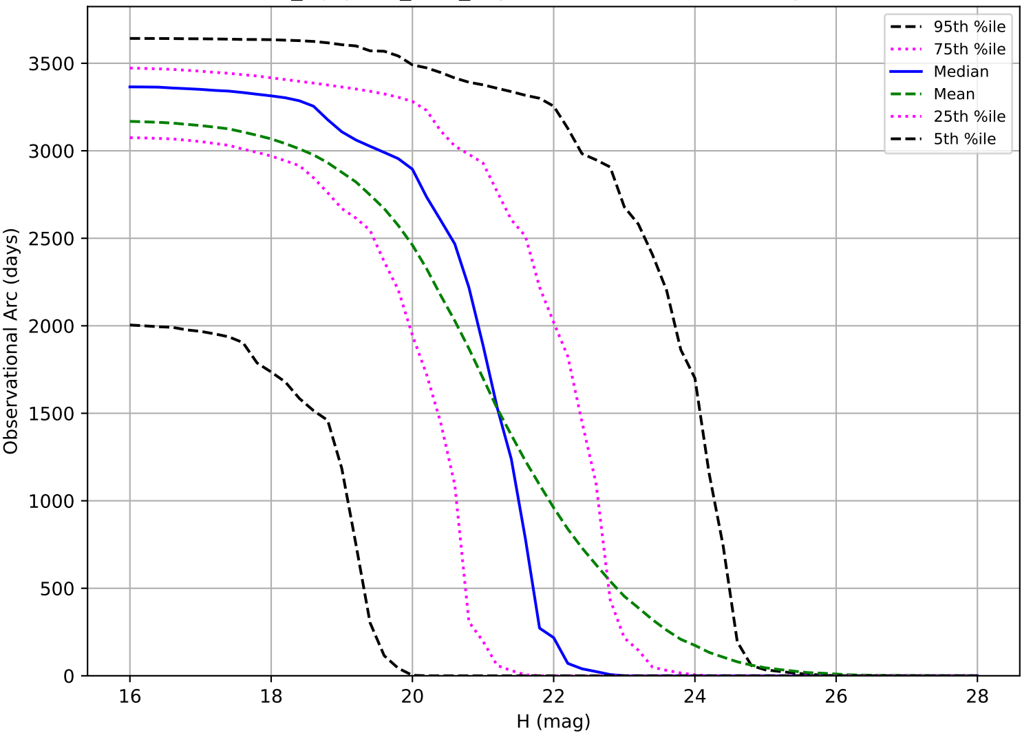
noroll_mjdp120_v3.4_10yrs: Observational Arc Length PHA
