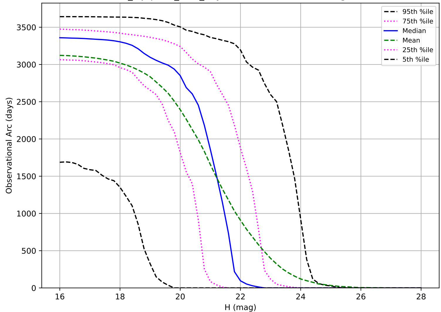
noroll_mjdp120_v3.4_10yrs: Observational Arc Length NEO
