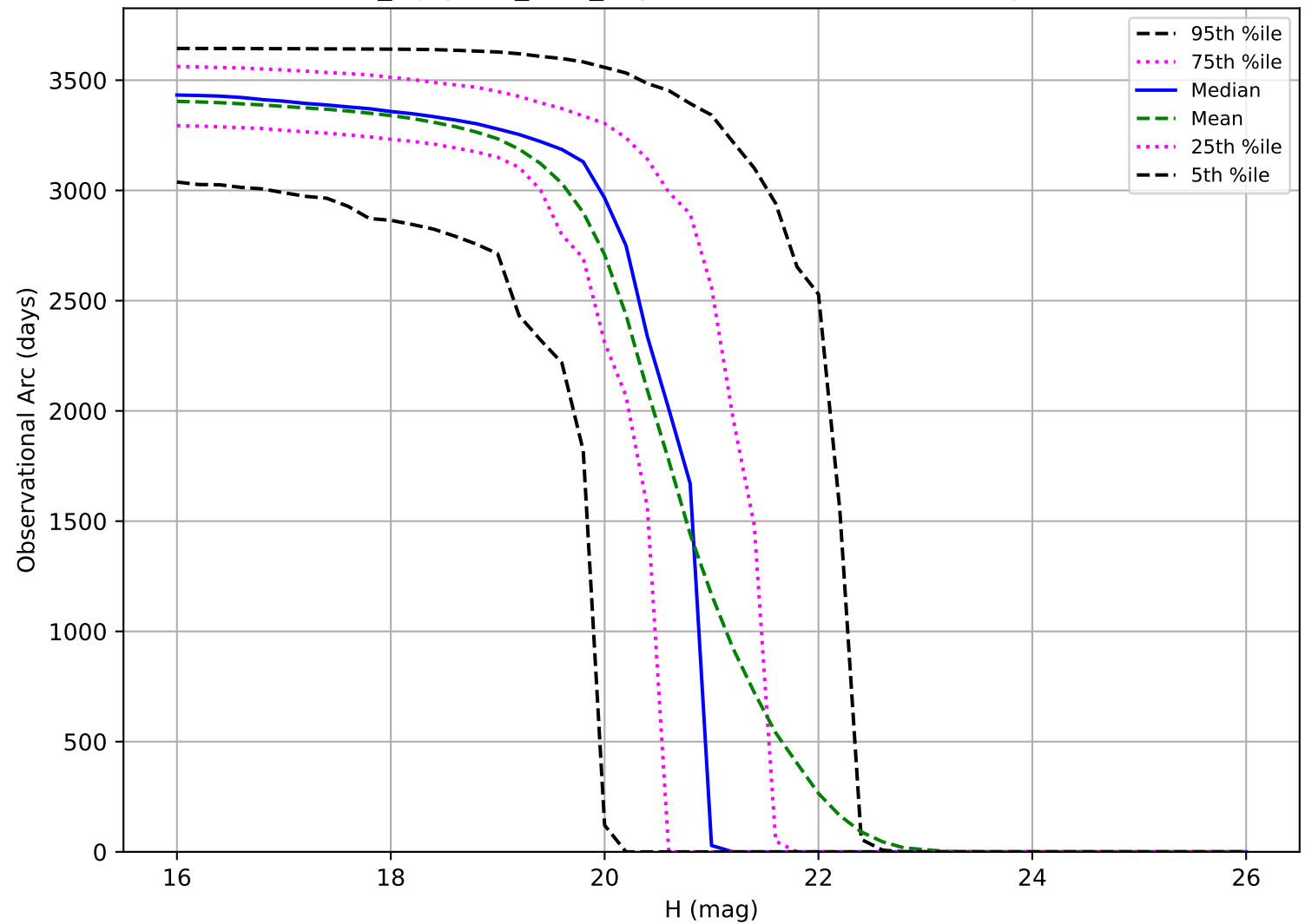
noroll_mjdp120_v3.4_10yrs: Observational Arc Length MBA
