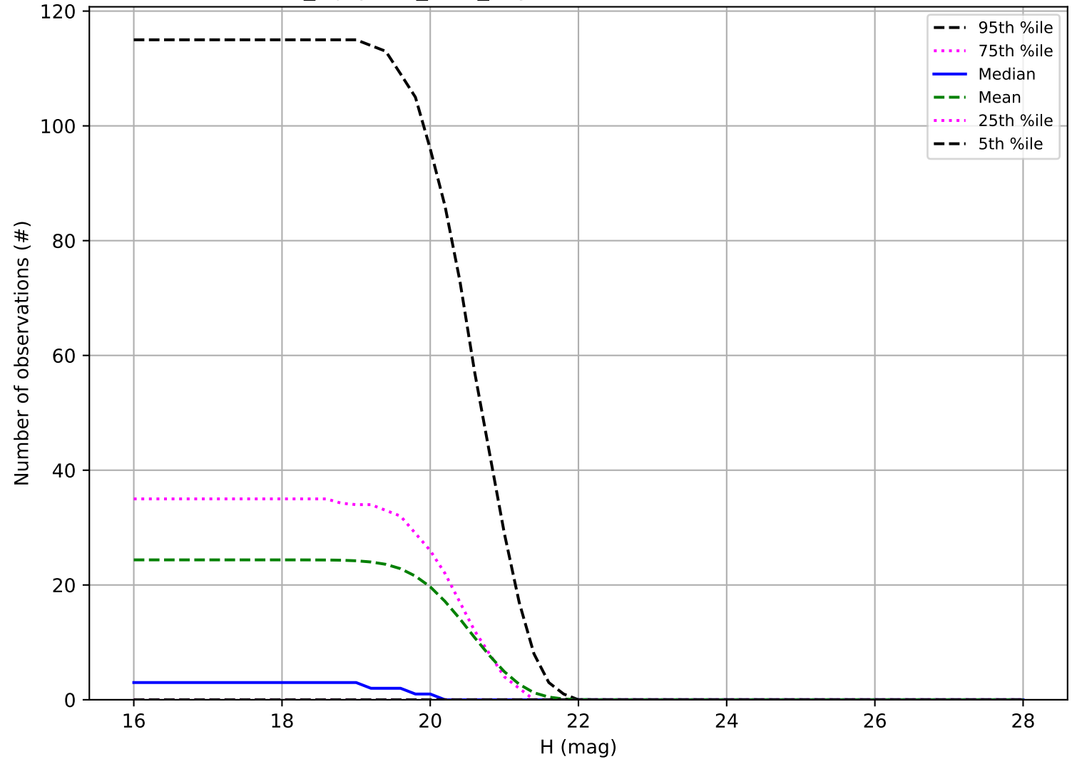
noroll_mjdp120_v3.4_10yrs: Number of observations Vatira
