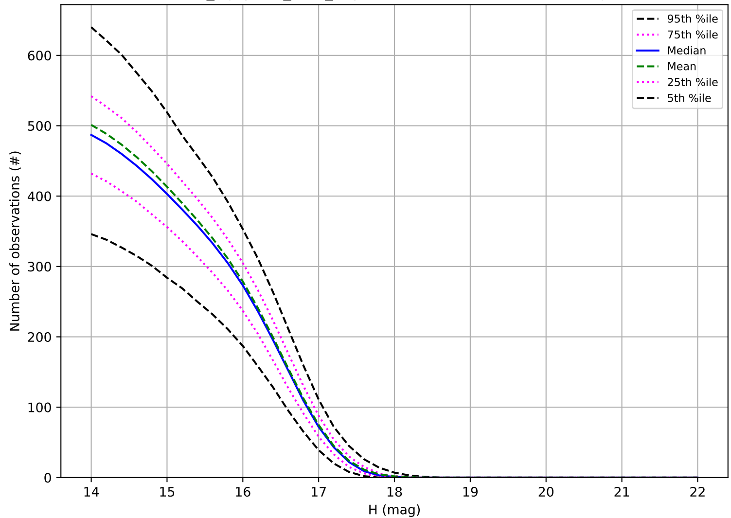
noroll_mjdp120_v3.4_10yrs: Number of observations Trojan
