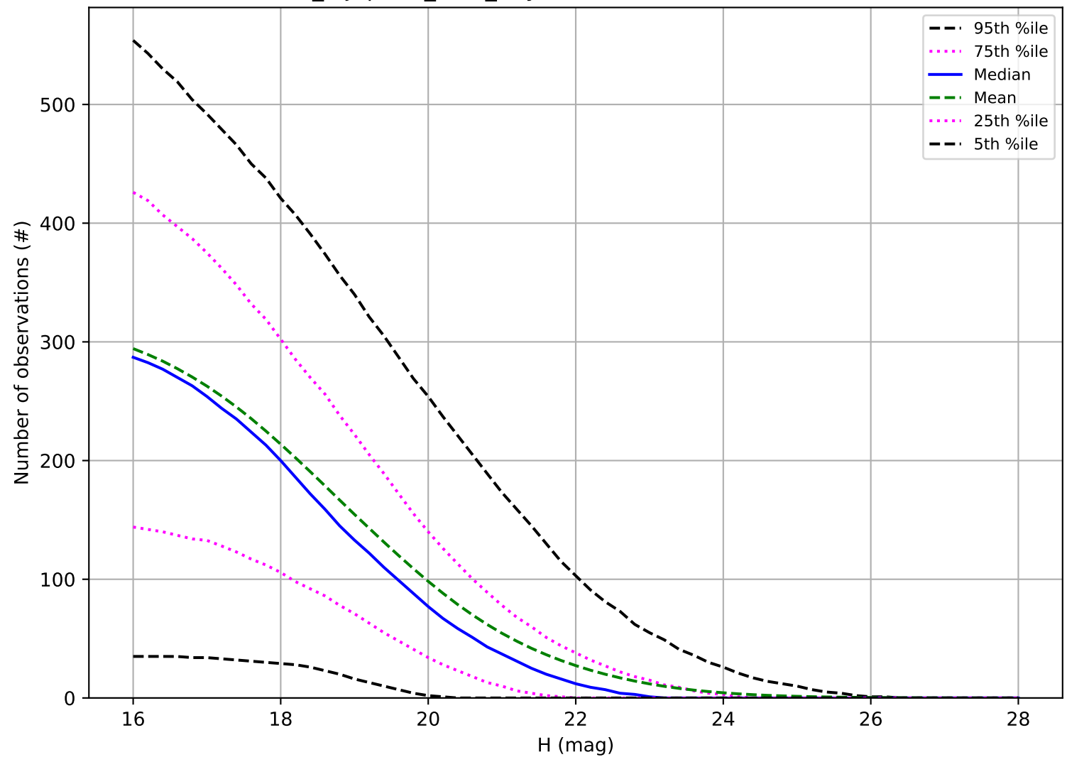
noroll_mjdp120_v3.4_10yrs: Number of observations PHA
