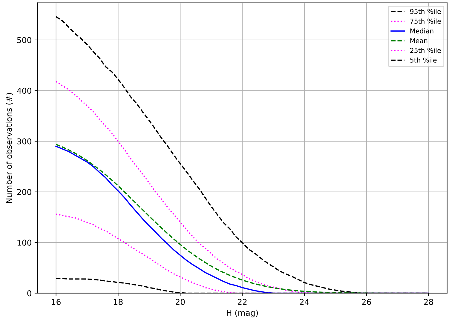
noroll_mjdp120_v3.4_10yrs: Number of observations NEO
