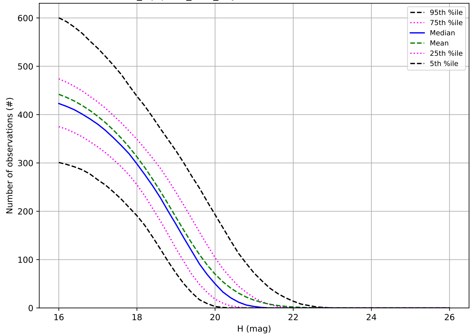
noroll_mjdp120_v3.4_10yrs: Number of observations MBA
