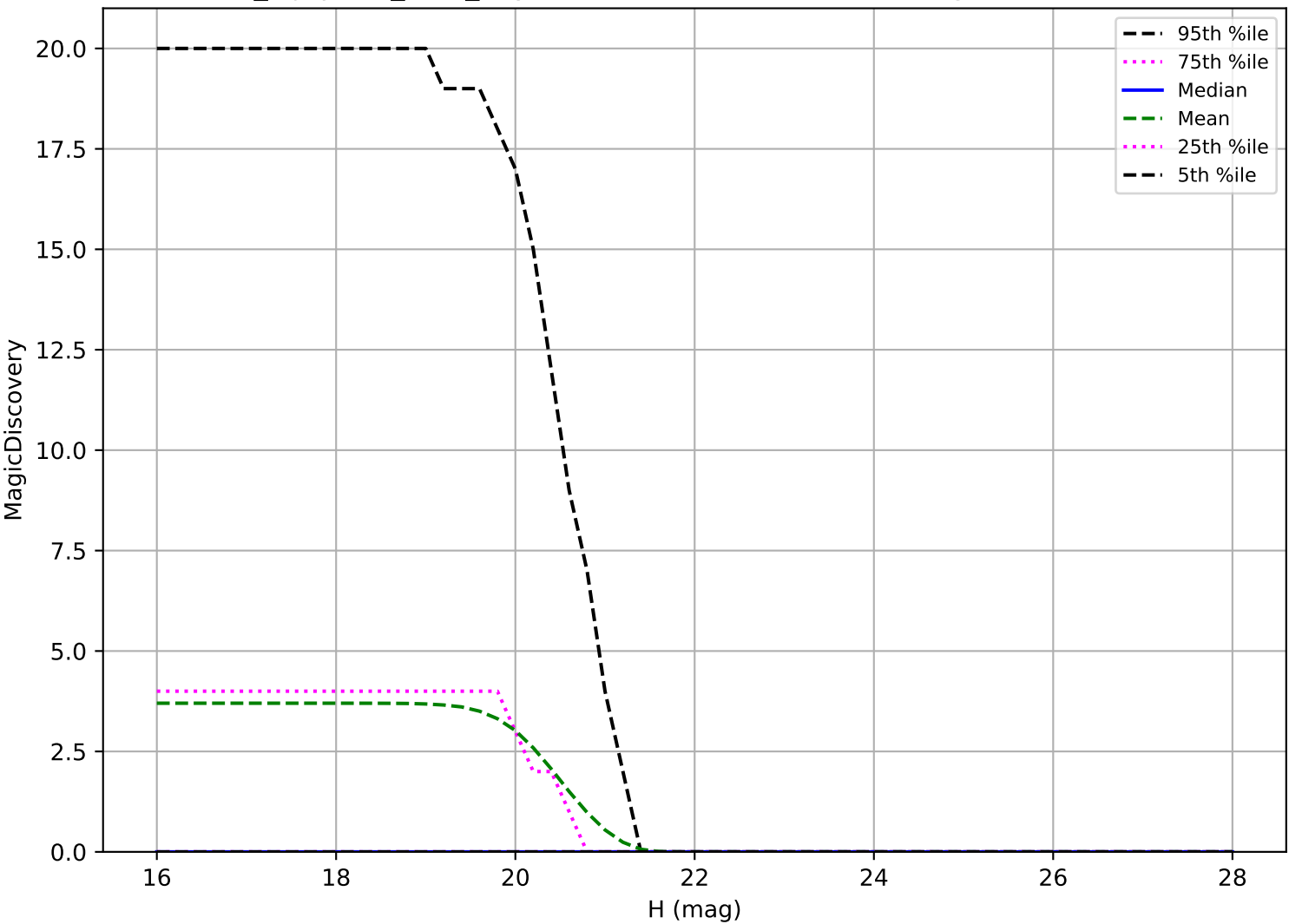
noroll_mjdp120_v3.4_10yrs: Vatira 6 detections in 60 nights detection loss
