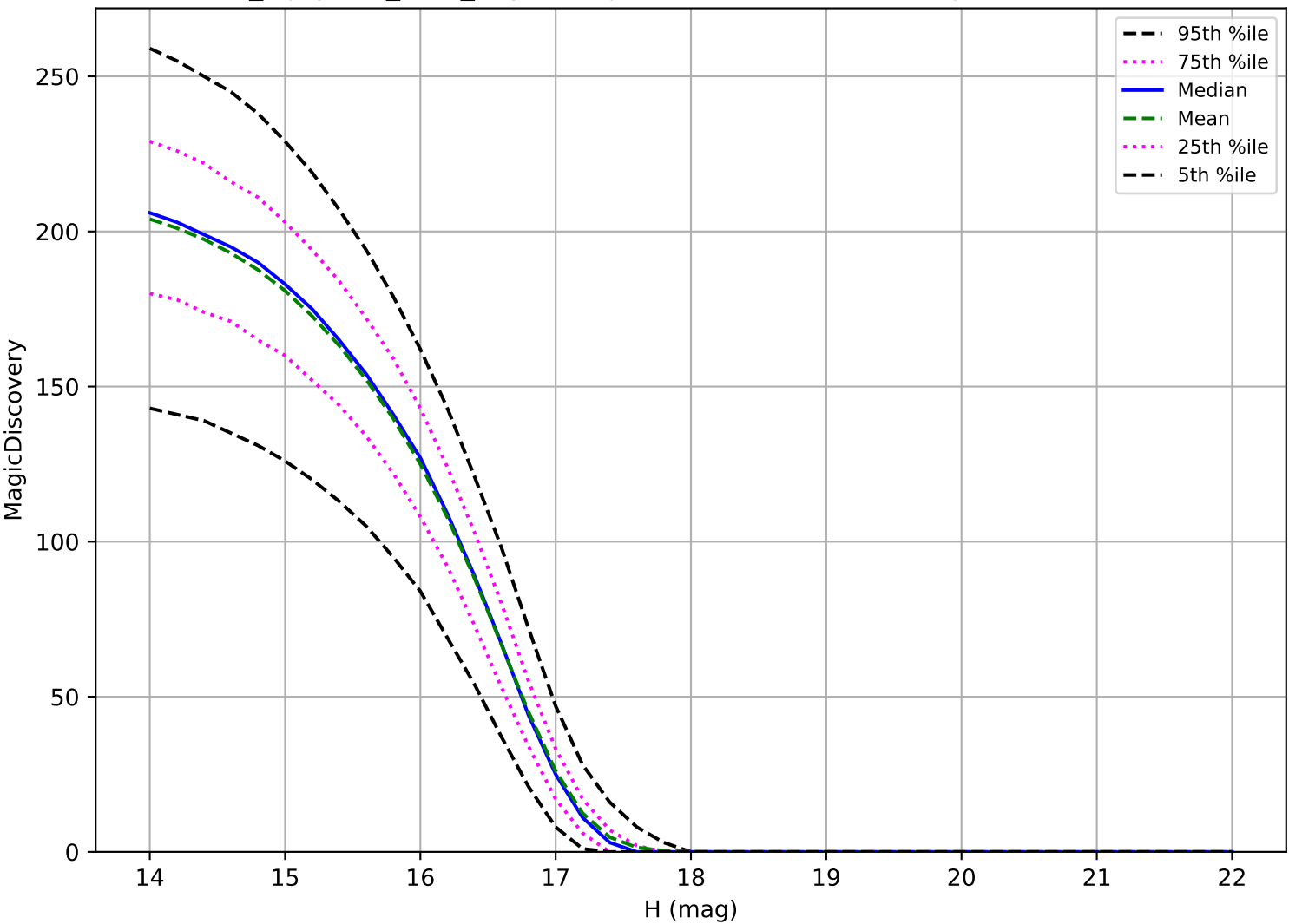
noroll_mjdp120_v3.4_10yrs: Trojan 6 detections in 60 nights detection loss
