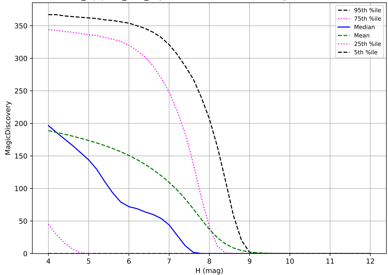
noroll_mjdp120_v3.4_10yrs: TNO 6 detections in 60 nights detection loss
