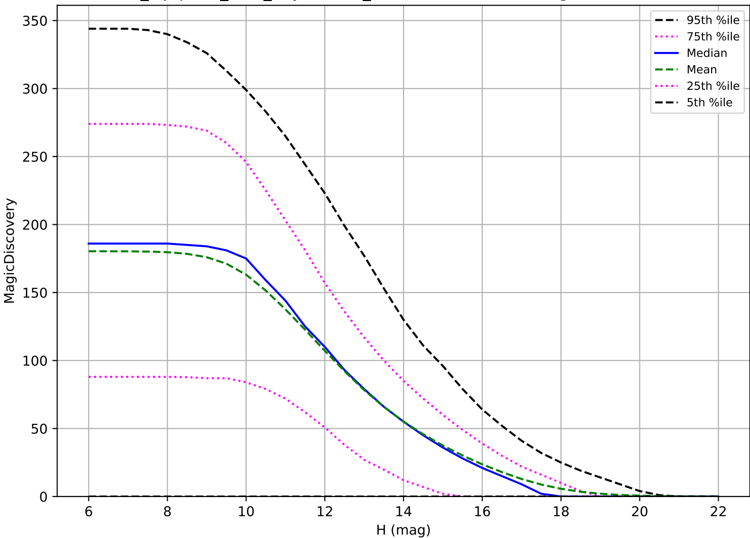
noroll_mjdp120_v3.4_10yrs: OCC_r5 6 detections in 60 nights detection loss
