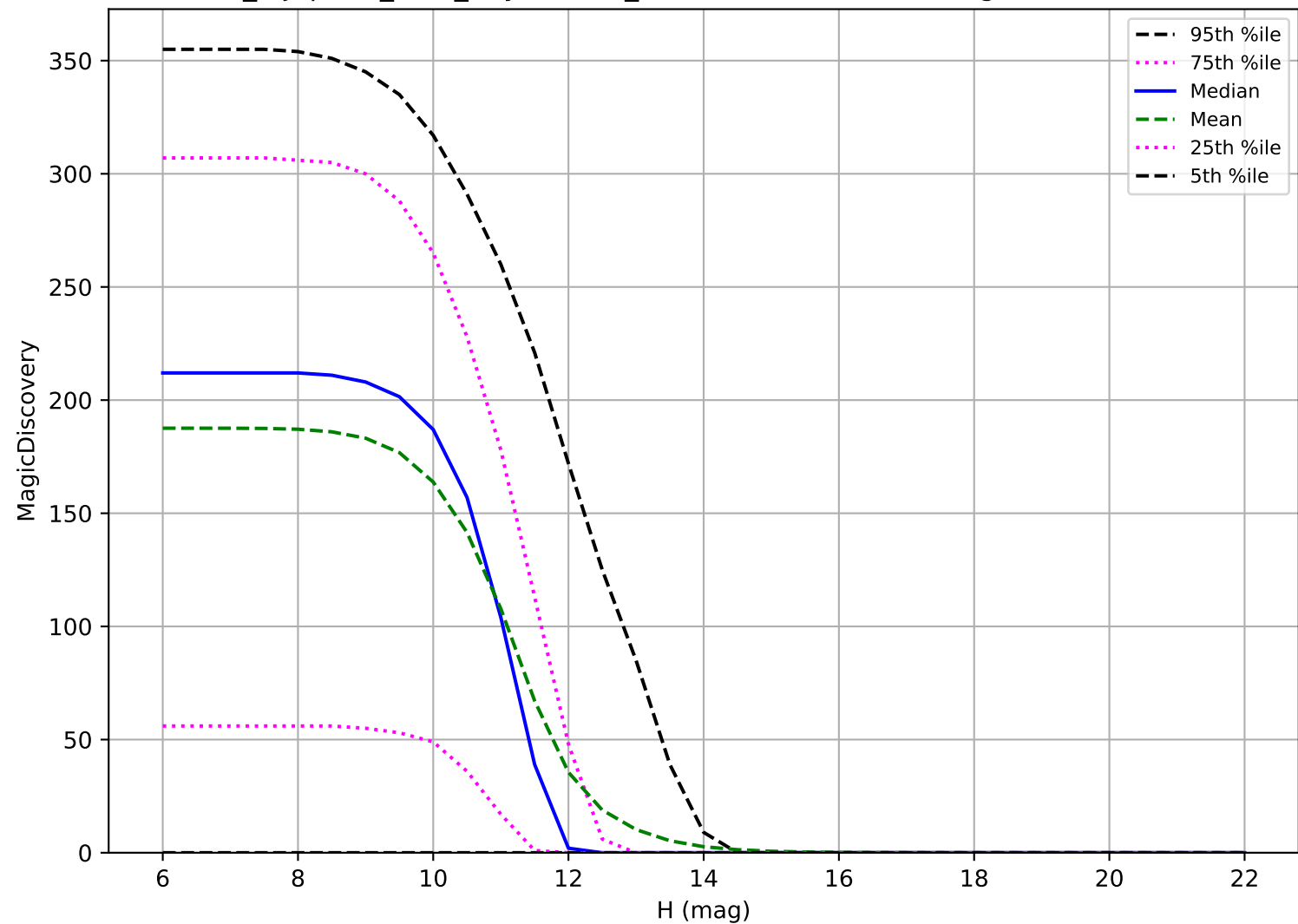
noroll_mjdp120_v3.4_10yrs: OCC_r20 6 detections in 60 nights detection loss
