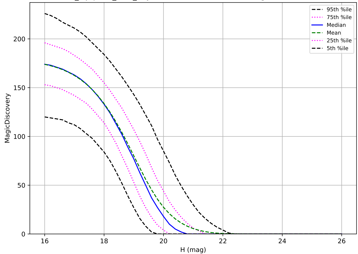
noroll_mjdp120_v3.4_10yrs: MBA 6 detections in 60 nights detection loss
