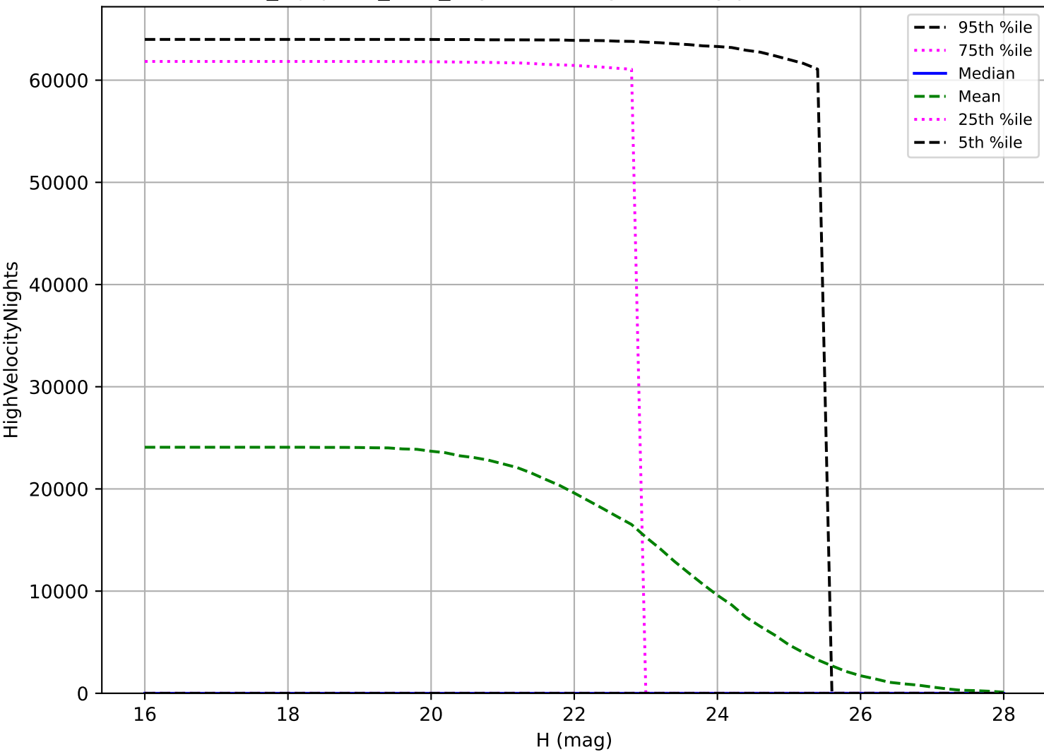
noroll_mjdp120_v3.4_10yrs: PHA High velocity pair detection loss
