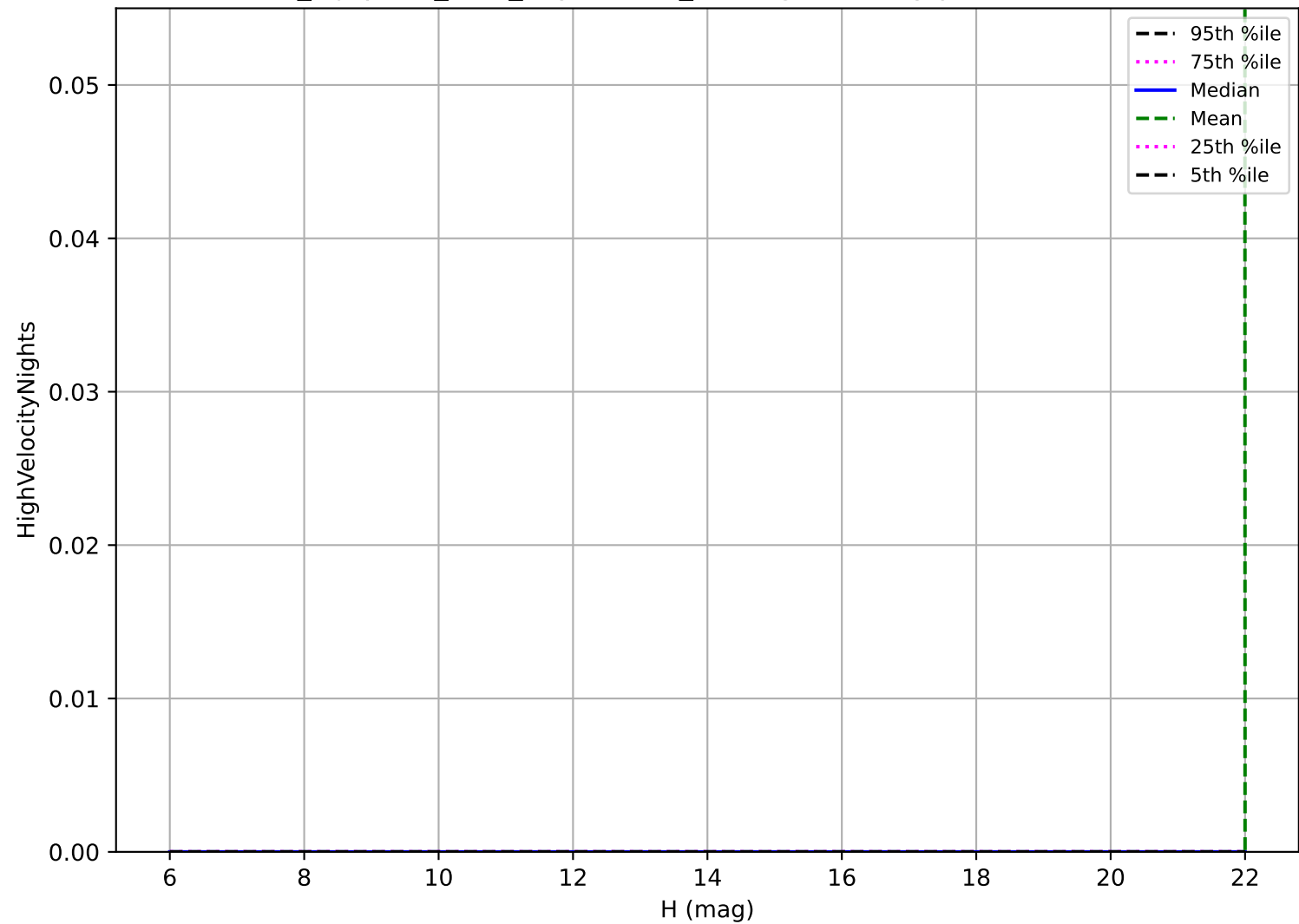
noroll_mjdp120_v3.4_10yrs: OCC_r20 High velocity pair detection loss
