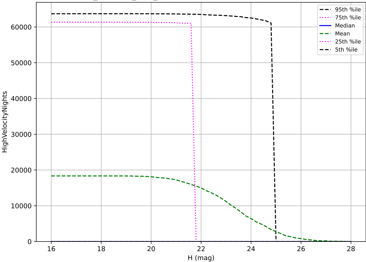
noroll_mjdp120_v3.4_10yrs: NEO High velocity pair detection loss
