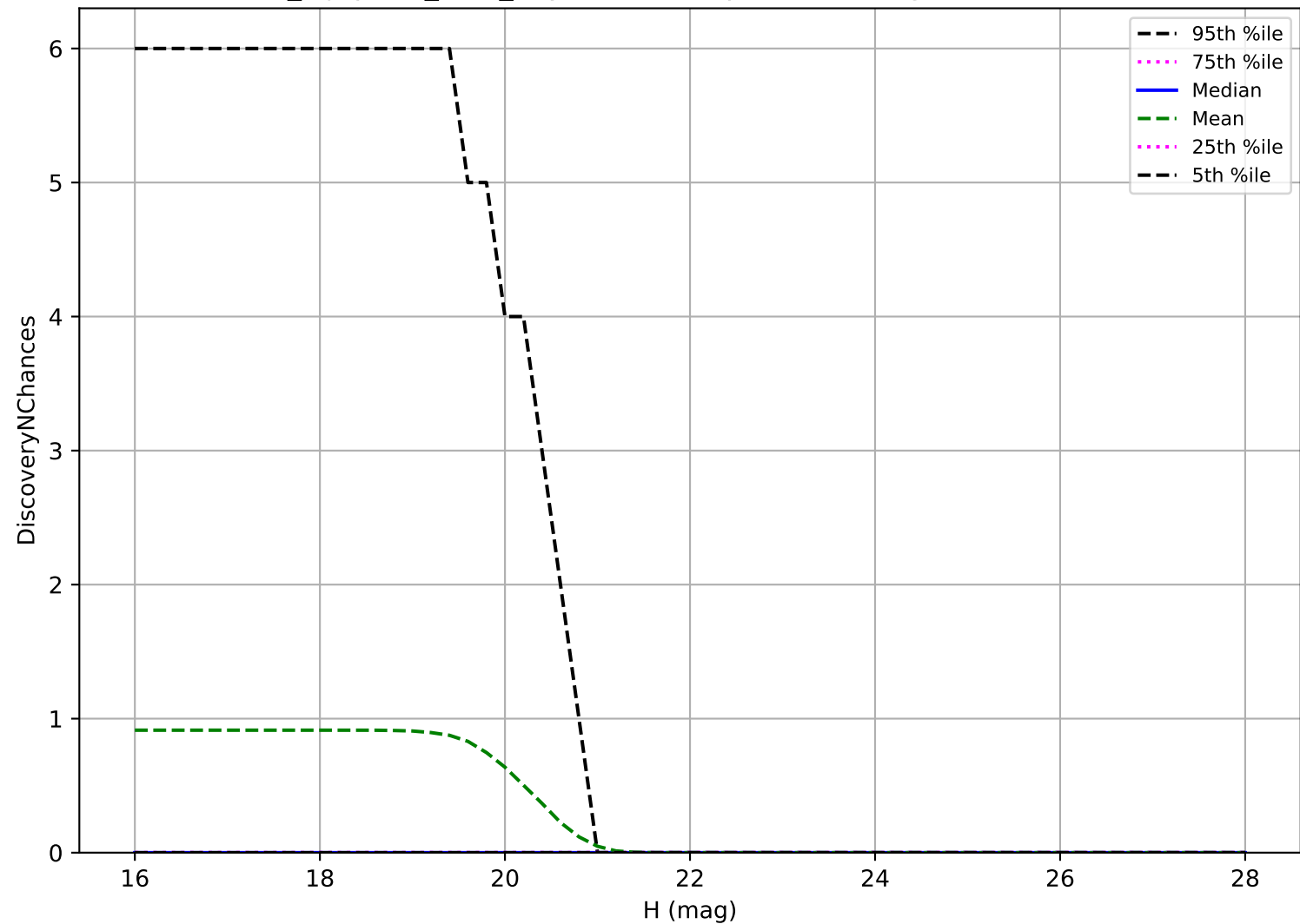
noroll_mjdp120_v3.4_10yrs: Vatira 3 pairs in 15 nights detection loss
