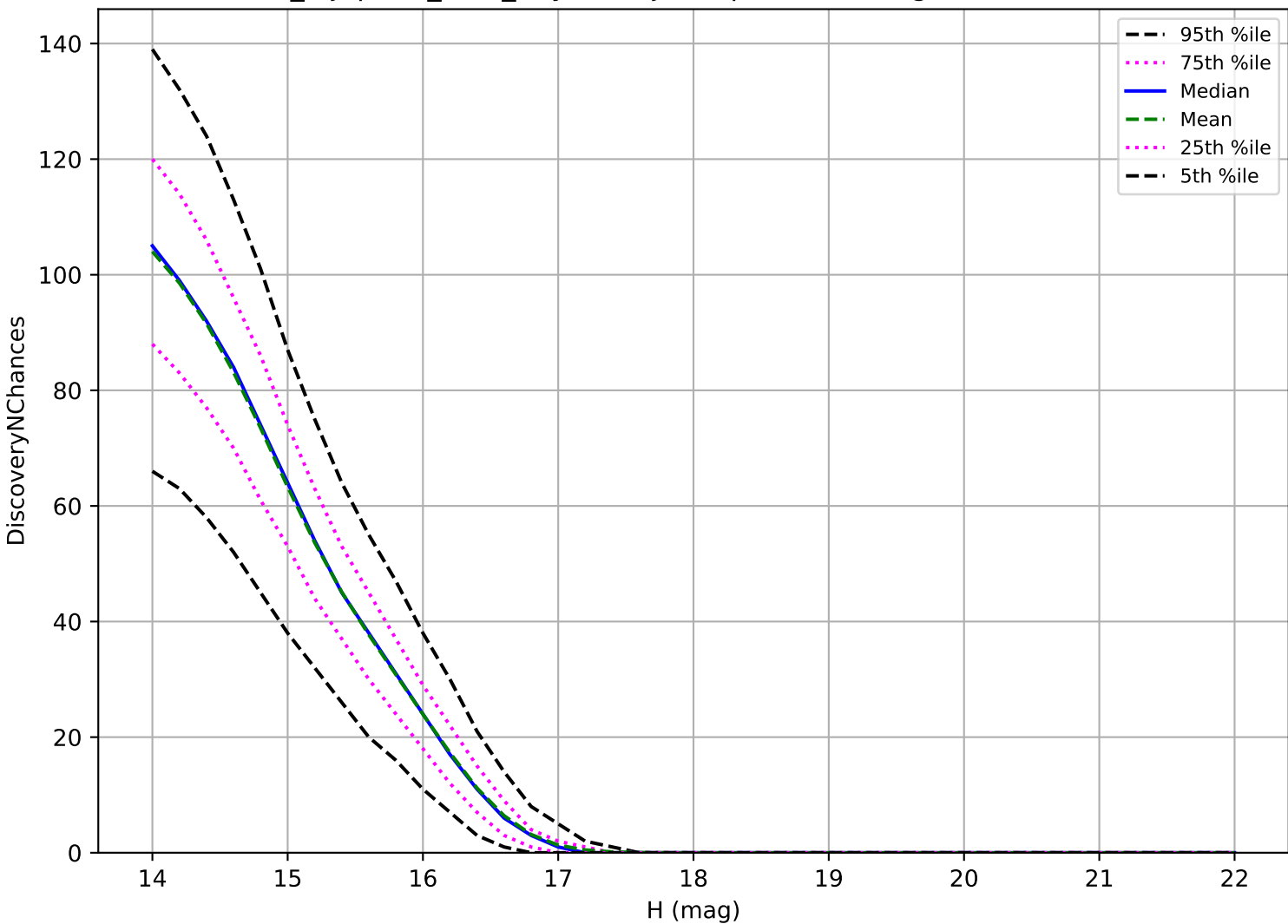
noroll_mjdp120_v3.4_10yrs: Trojan 3 pairs in 15 nights detection loss
