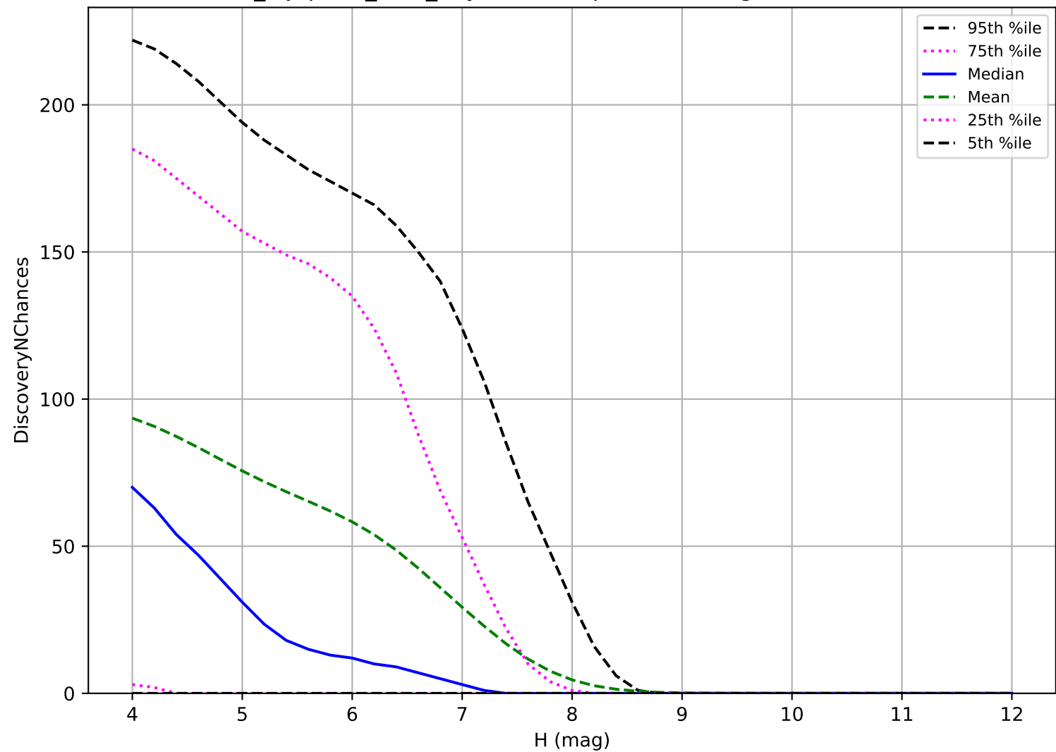
noroll_mjdp120_v3.4_10yrs: TNO 3 pairs in 15 nights detection loss
