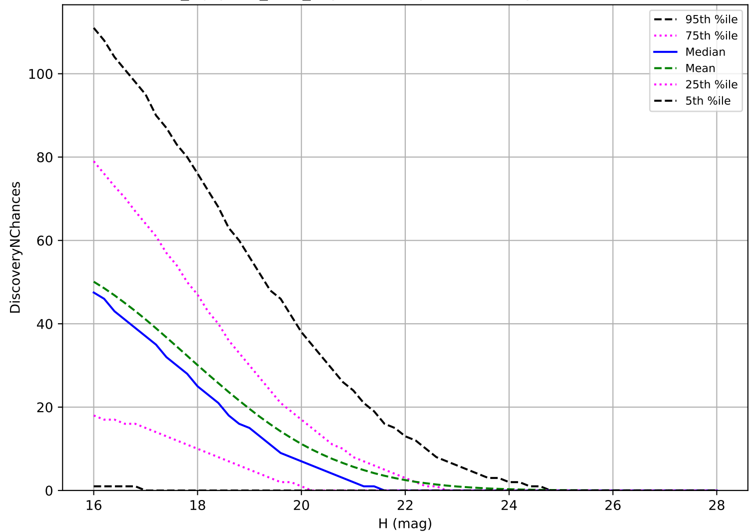
noroll_mjdp120_v3.4_10yrs: PHA 3 pairs in 15 nights detection loss
