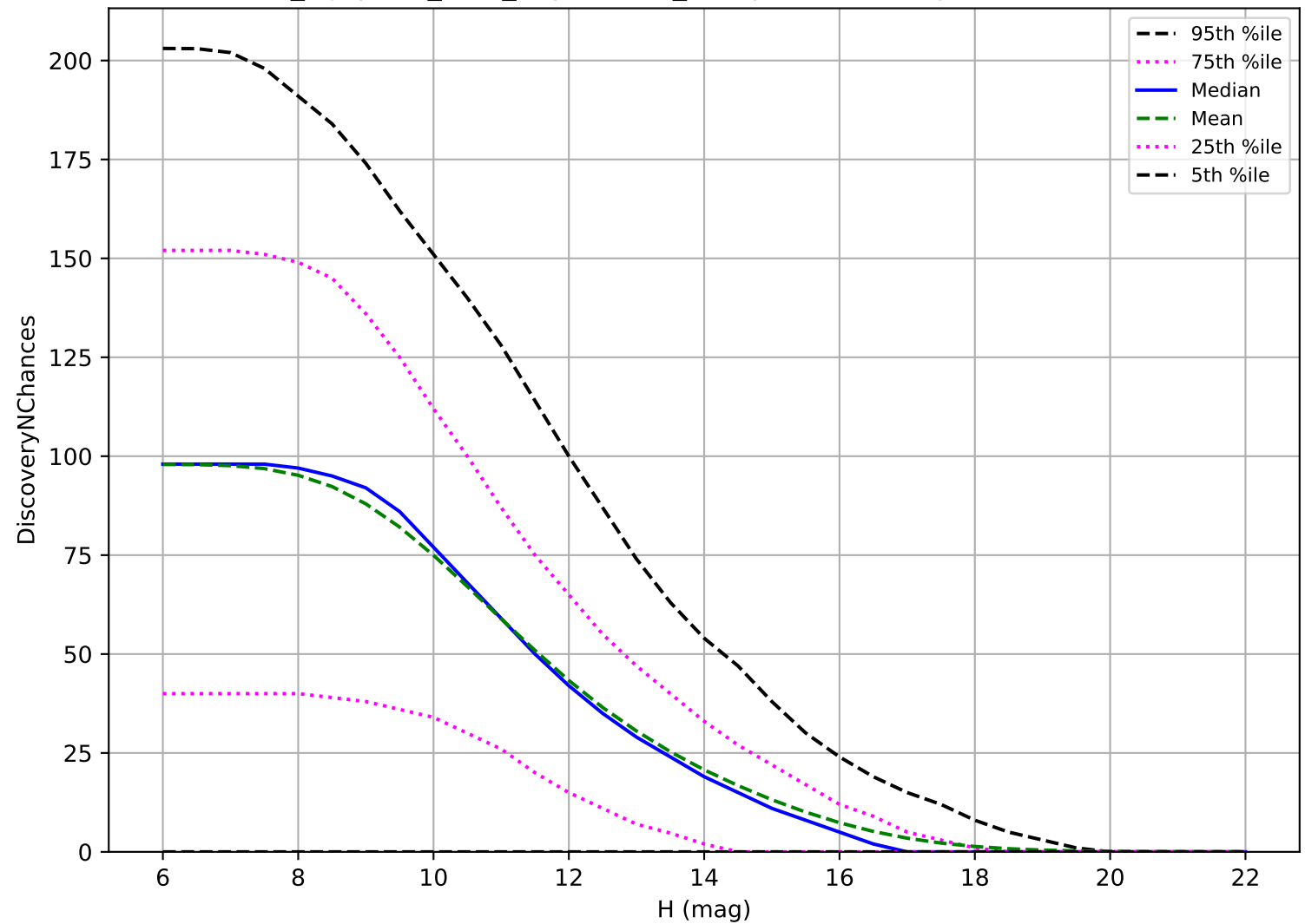
noroll_mjdp120_v3.4_10yrs: OCC_r5 3 pairs in 15 nights detection loss
