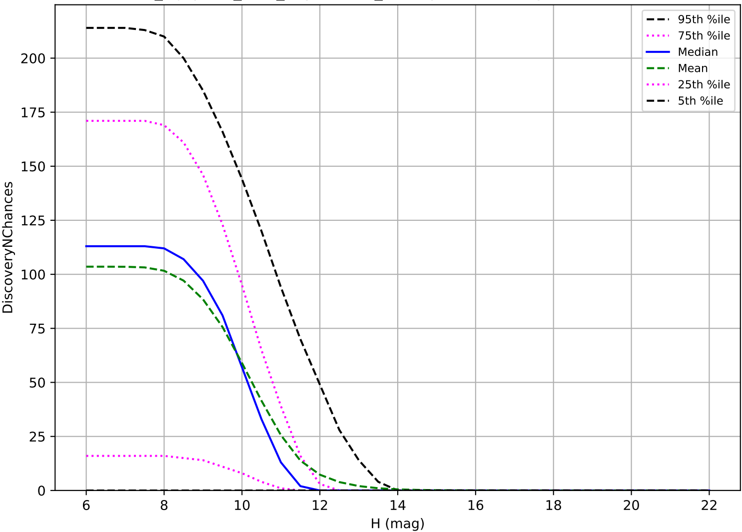
noroll_mjdp120_v3.4_10yrs: OCC_r20 3 pairs in 15 nights detection loss
