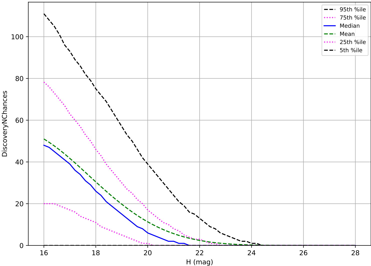
noroll_mjdp120_v3.4_10yrs: NEO 3 pairs in 15 nights detection loss
