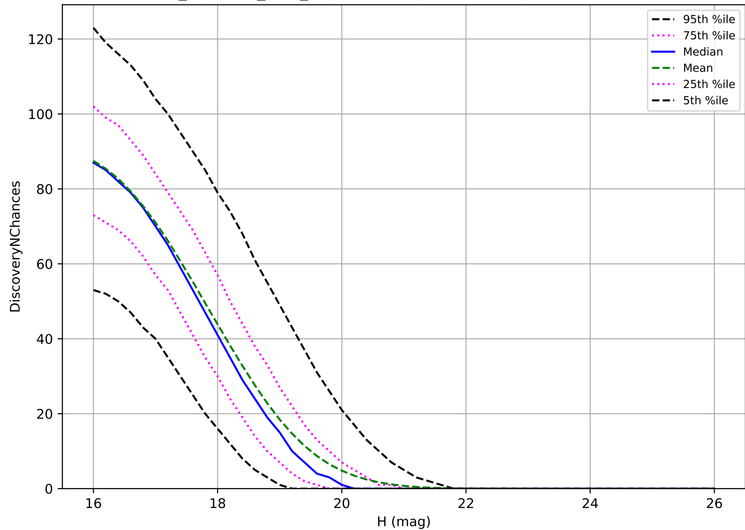
noroll_mjdp120_v3.4_10yrs: MBA 3 pairs in 15 nights detection loss
