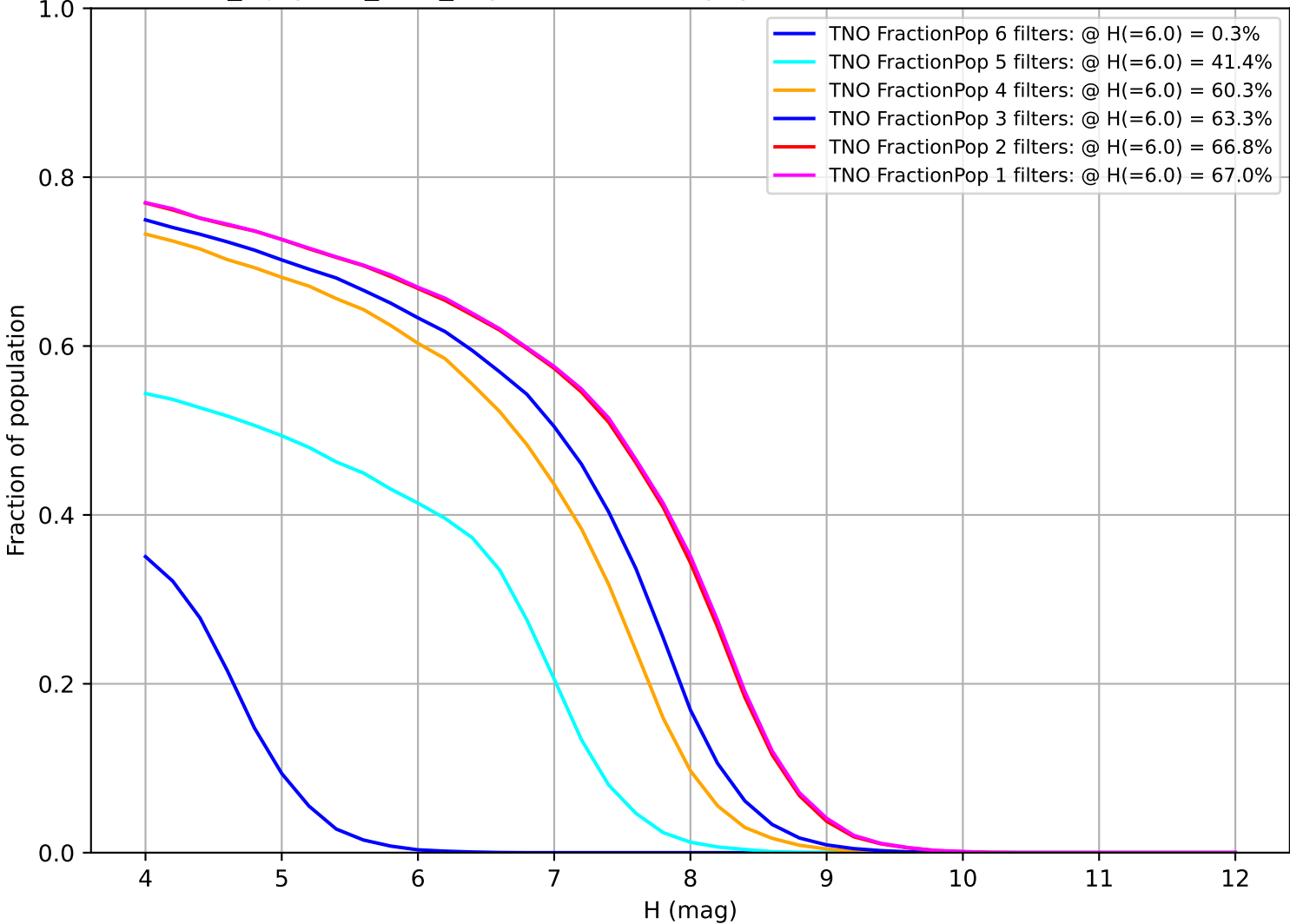
noroll_mjdp120_v3.4_10yrs: Fraction of population with colors in X filters TNO
