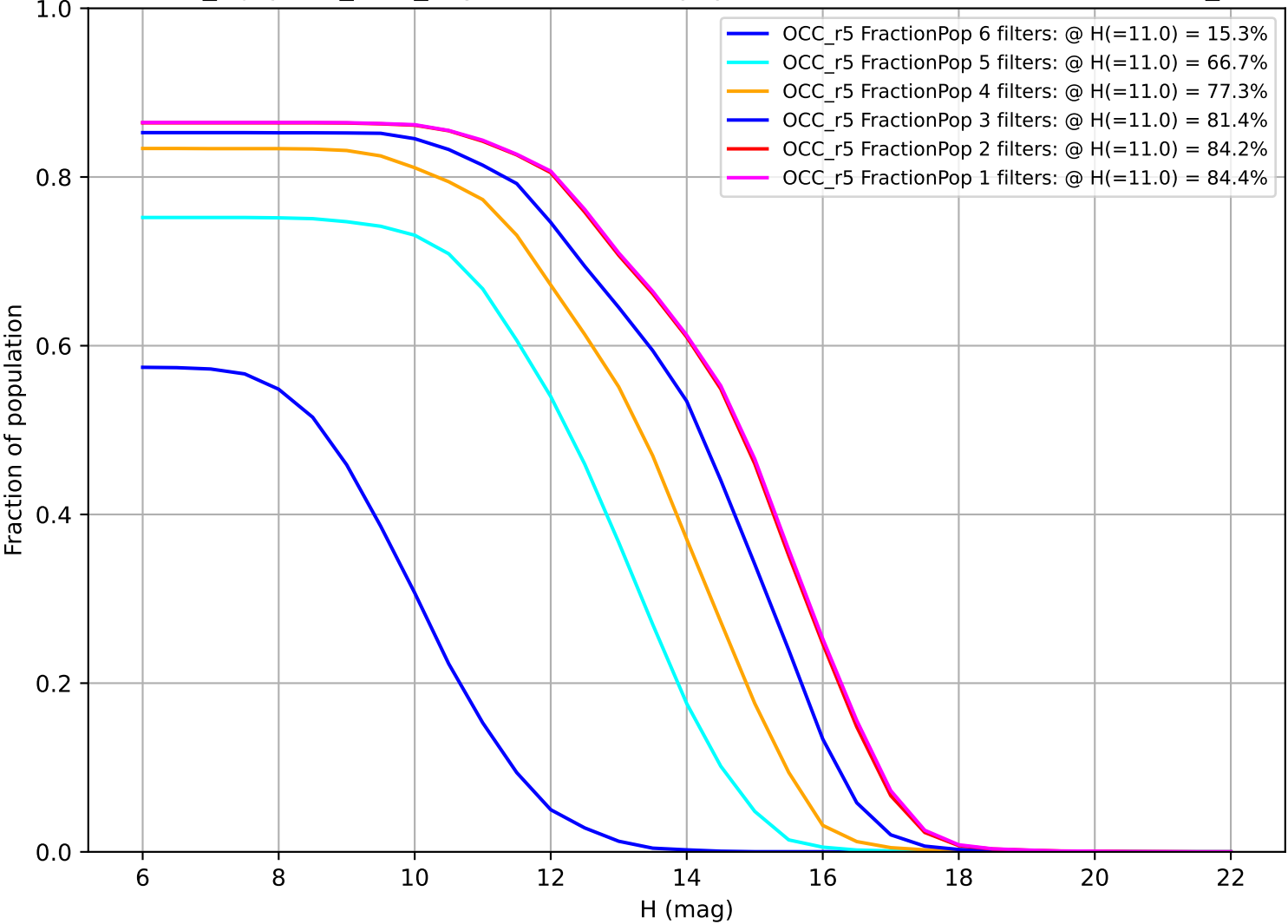
noroll_mjdp120_v3.4_10yrs: Fraction of population with colors in X filters OCC_r5
