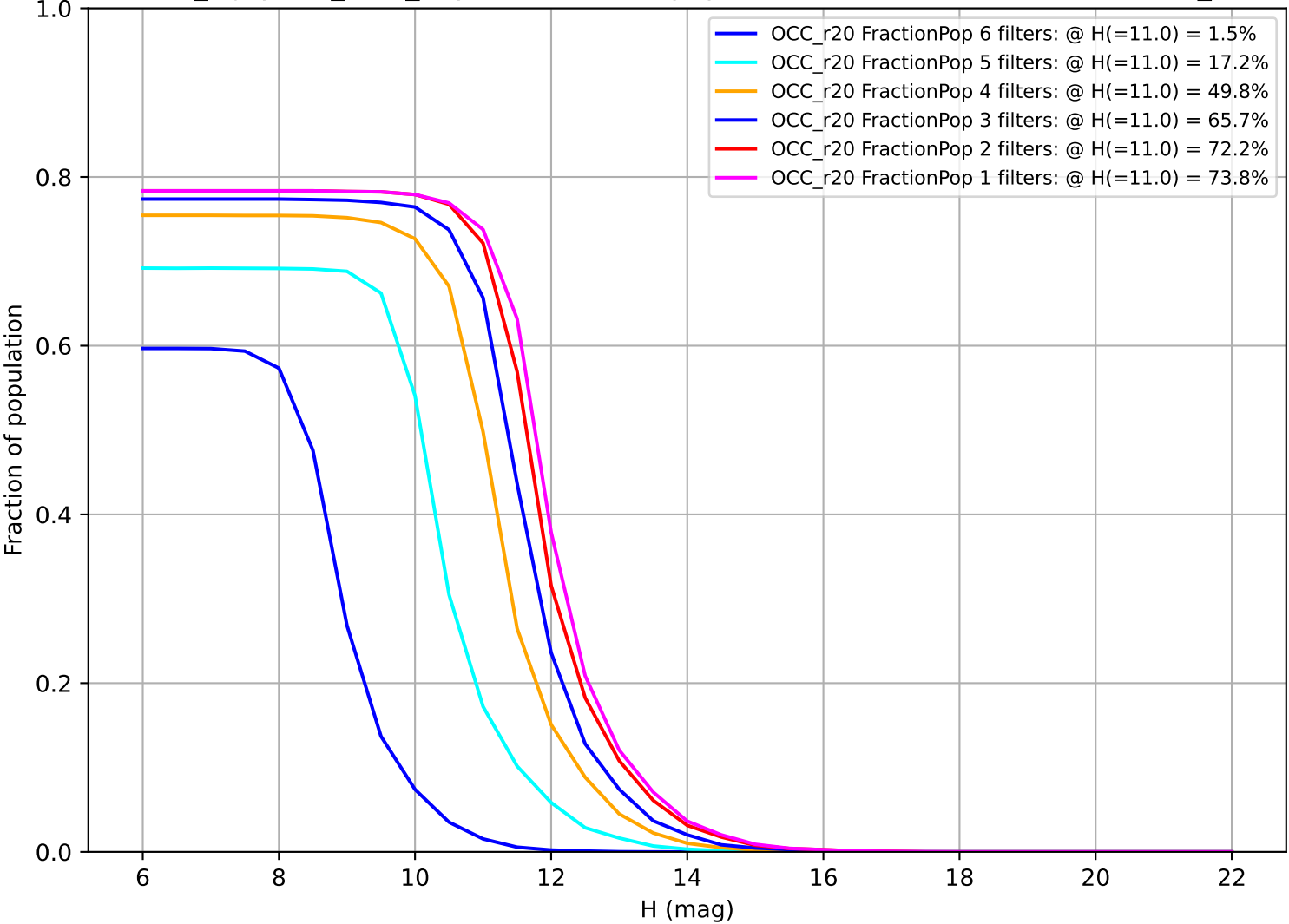
noroll_mjdp120_v3.4_10yrs: Fraction of population with colors in X filters OCC_r20
