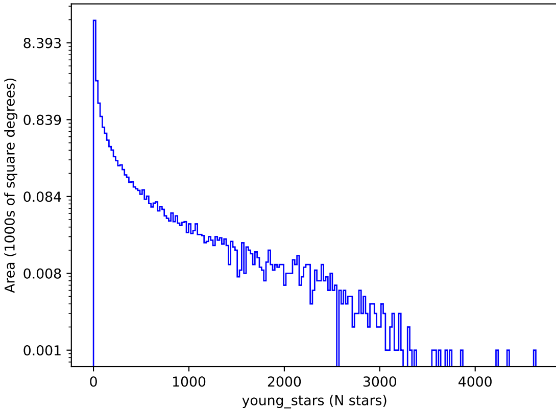
noroll_mjdp120_v3.4_10yrs : young_stars
