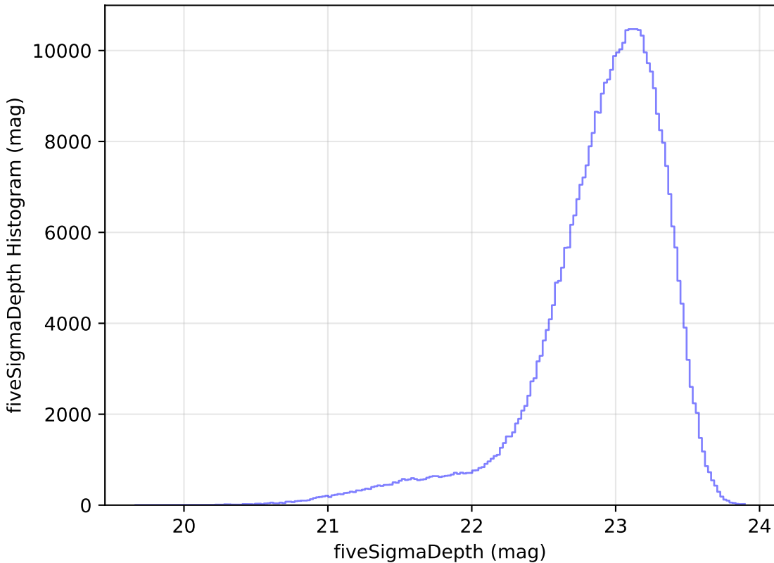
noroll_mjdp120_v3.4_10yrs z: fiveSigmaDepth Histogram
