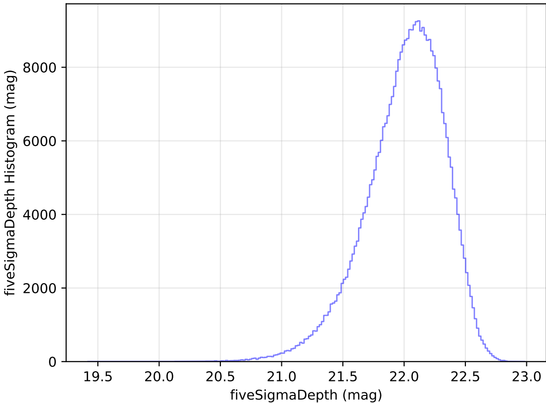
noroll_mjdp120_v3.4_10yrs y: fiveSigmaDepth Histogram
