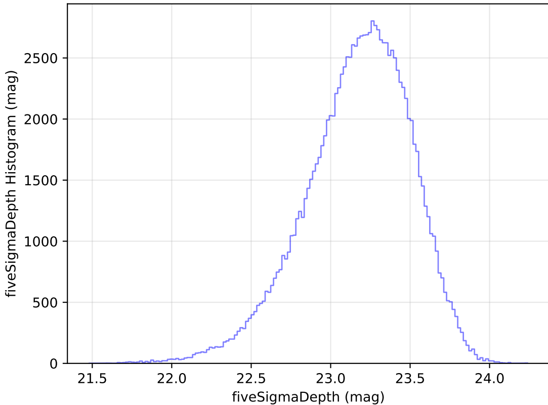
noroll_mjdp120_v3.4_10yrs u: fiveSigmaDepth Histogram
