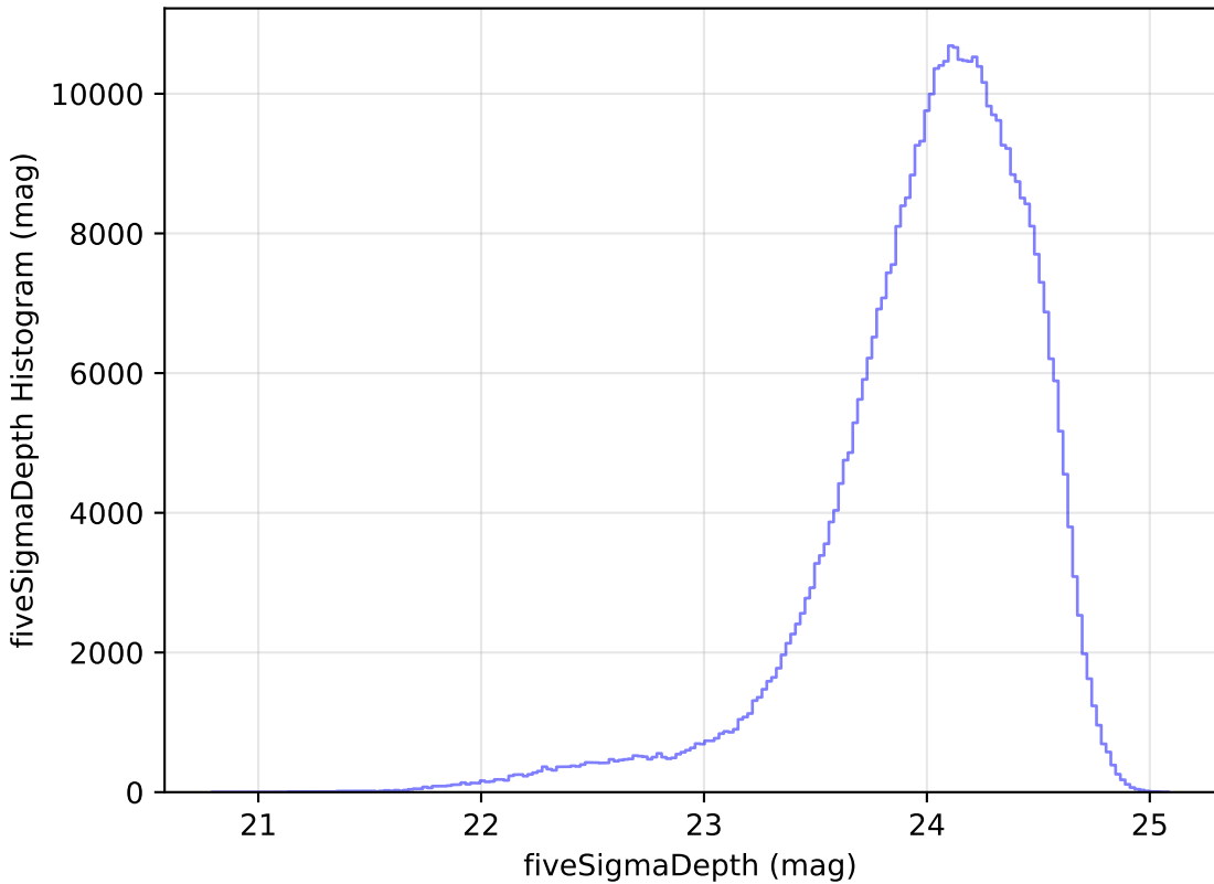
noroll_mjdp120_v3.4_10yrs r: fiveSigmaDepth Histogram
