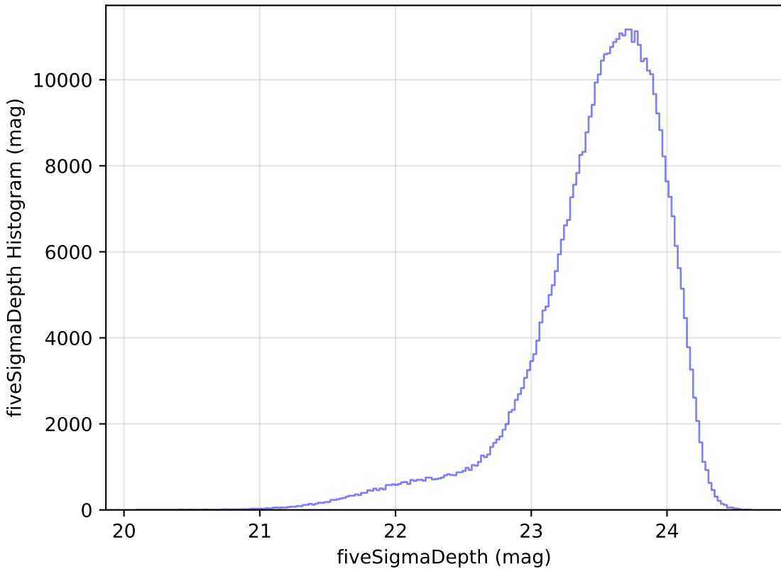
noroll_mjdp120_v3.4_10yrs i: fiveSigmaDepth Histogram
